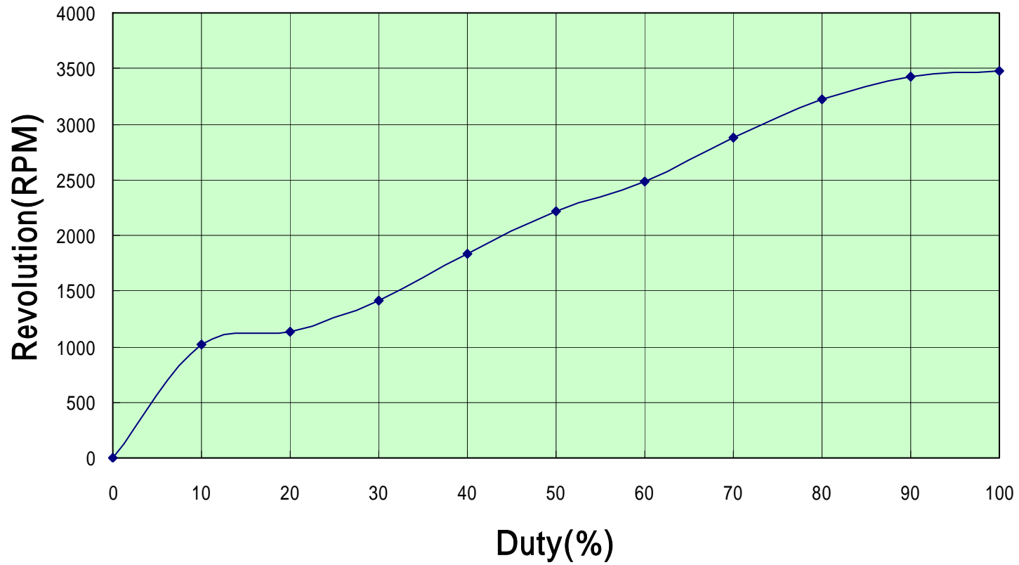
Aturbo PWM Curve
